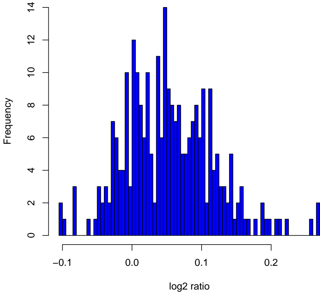
Histogram of log2ratios in 270 HapMap samples at clone Chr13tp-9E10
