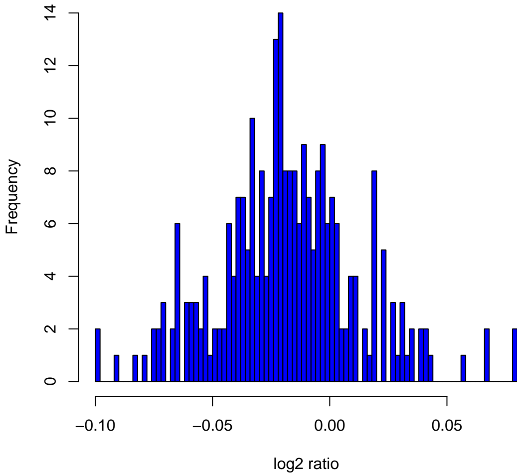
Histogram of log2ratios in 270 HapMap samples at clone Chr13tp-9G12
