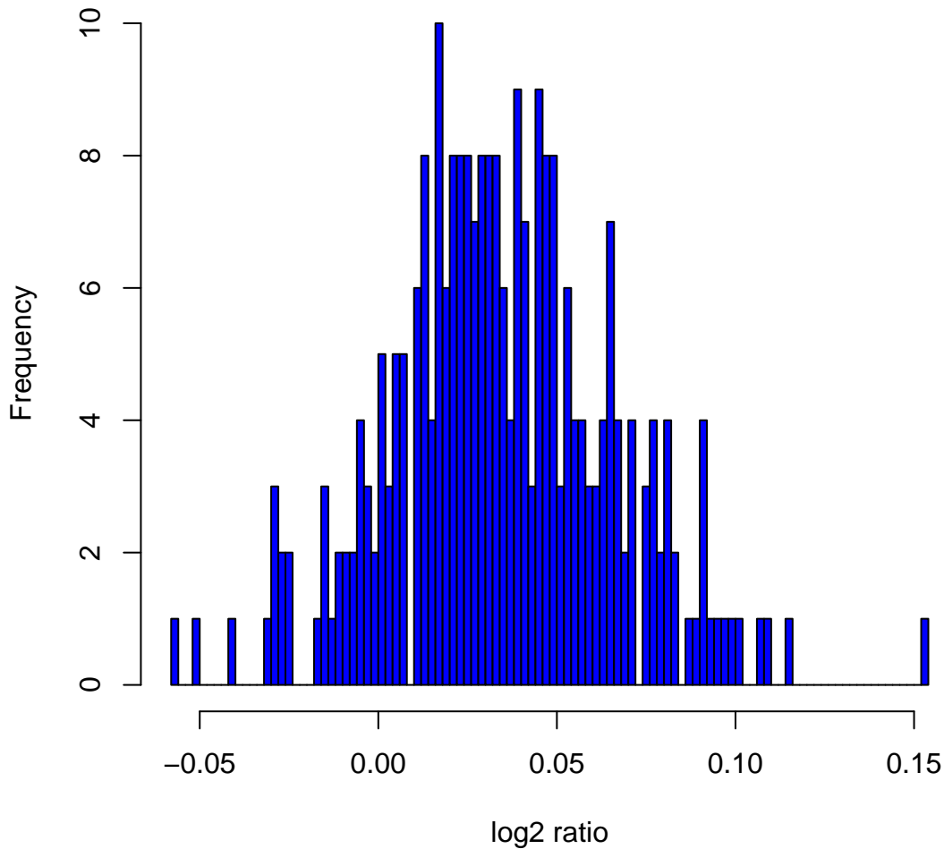
Histogram of log 2 ratios in 270 HapMap samples at clone Chr13tp-9G6
