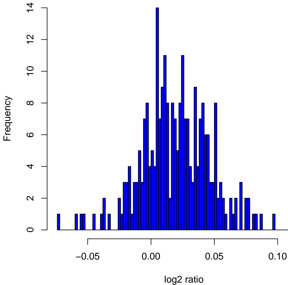
Histogram of log2ratios in 270 HapMap samples at clone Chr13tp-9H1
