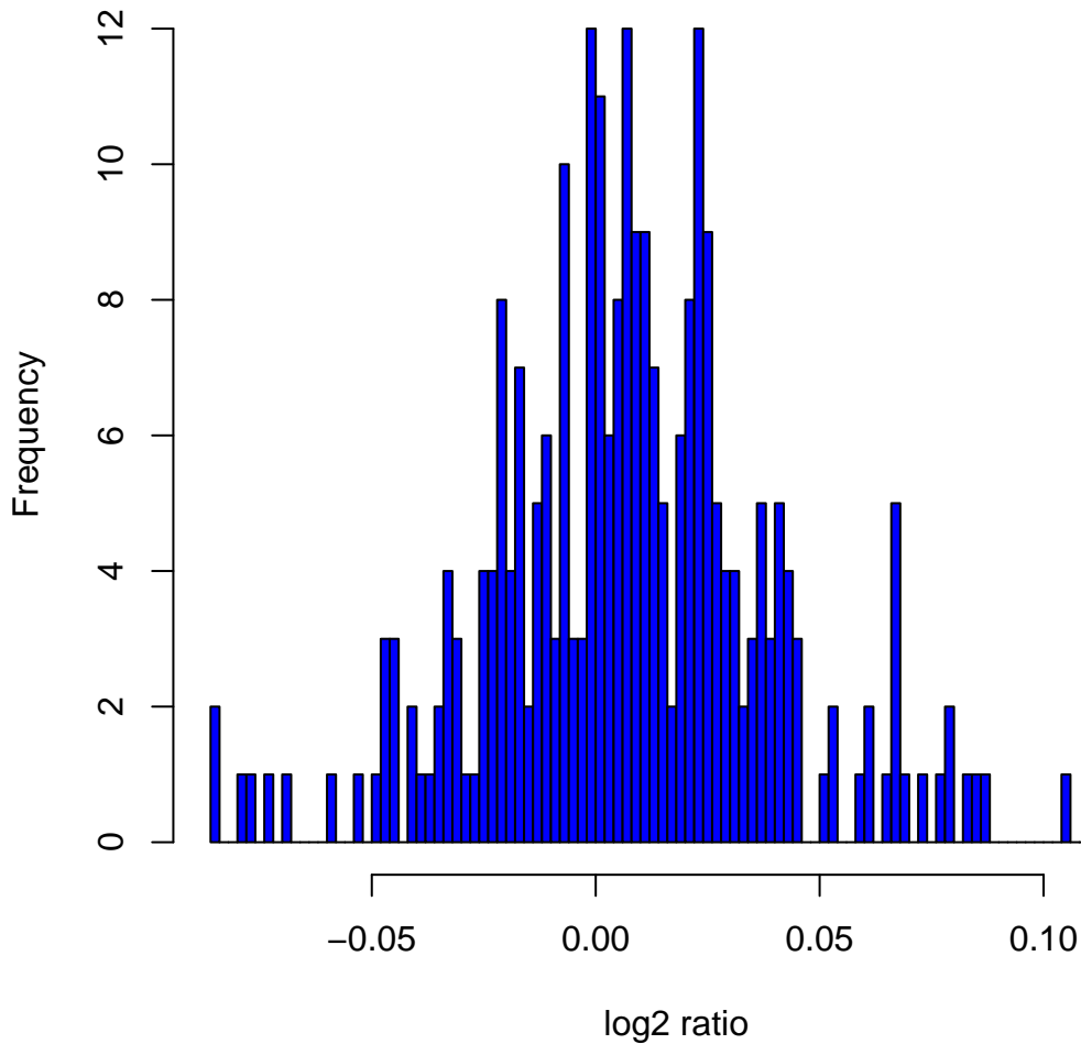
Histogram of log2ratios in 270 HapMap samples at clone Chr13tp-9H11
