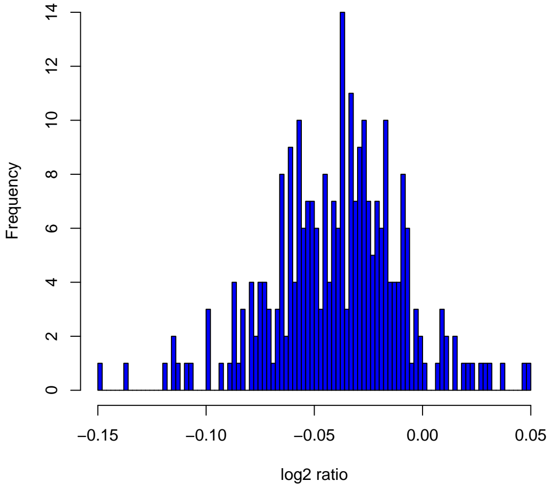
Histogram of log2ratios in 270 HapMap samples at clone Chr14tp-10A1
