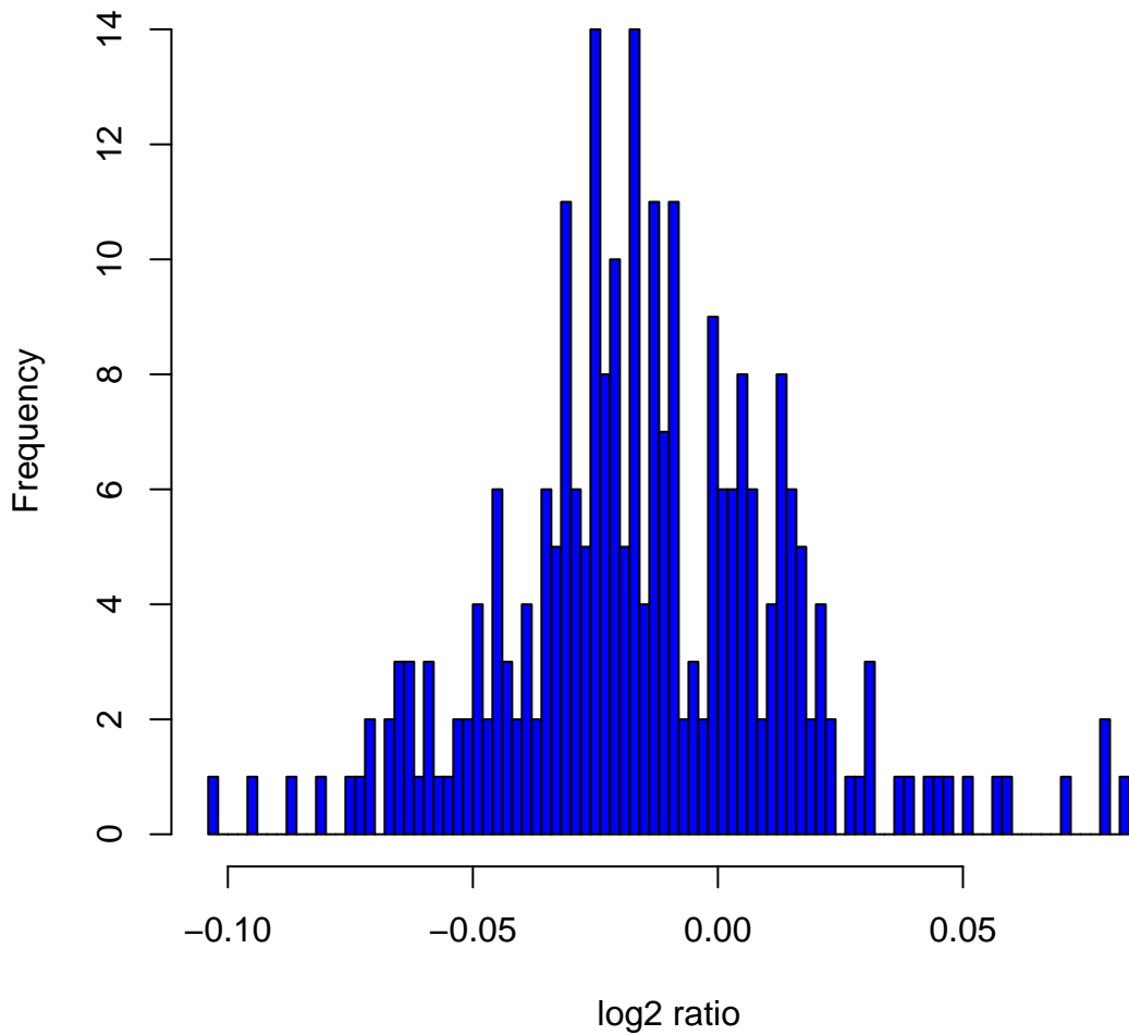
Histogram of log2ratios in 270 HapMap samples at clone Chr14tp-10B12
