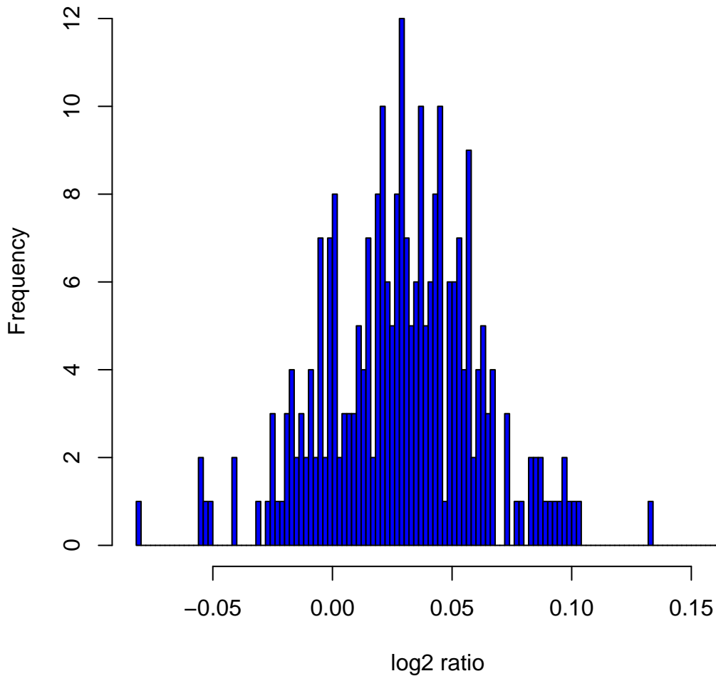
Histogram of log2ratios in 270 HapMap samples at clone Chr14tp-10G12
