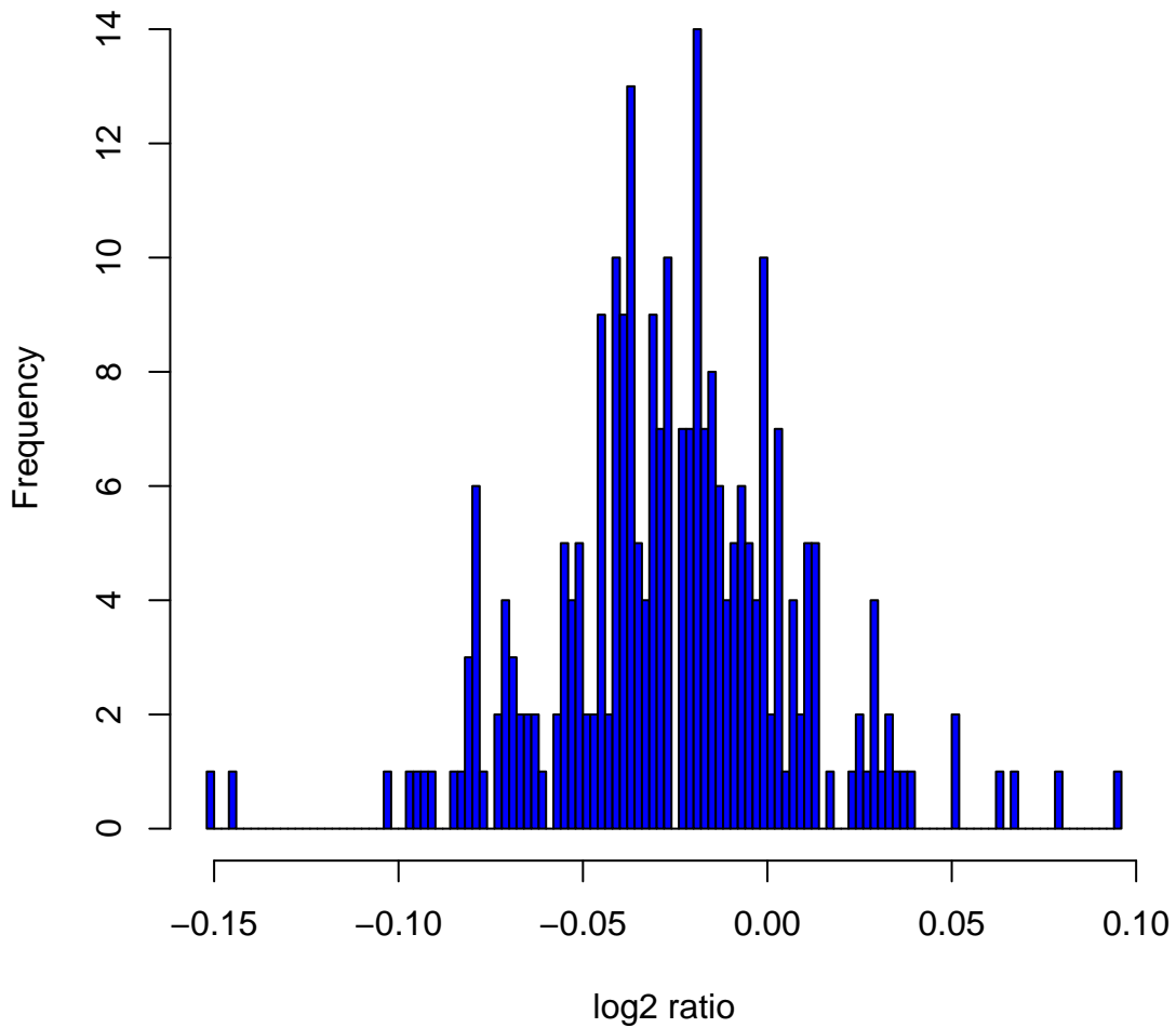
Histogram of log2ratios in 270 HapMap samples at clone Chr14tp-10H10
