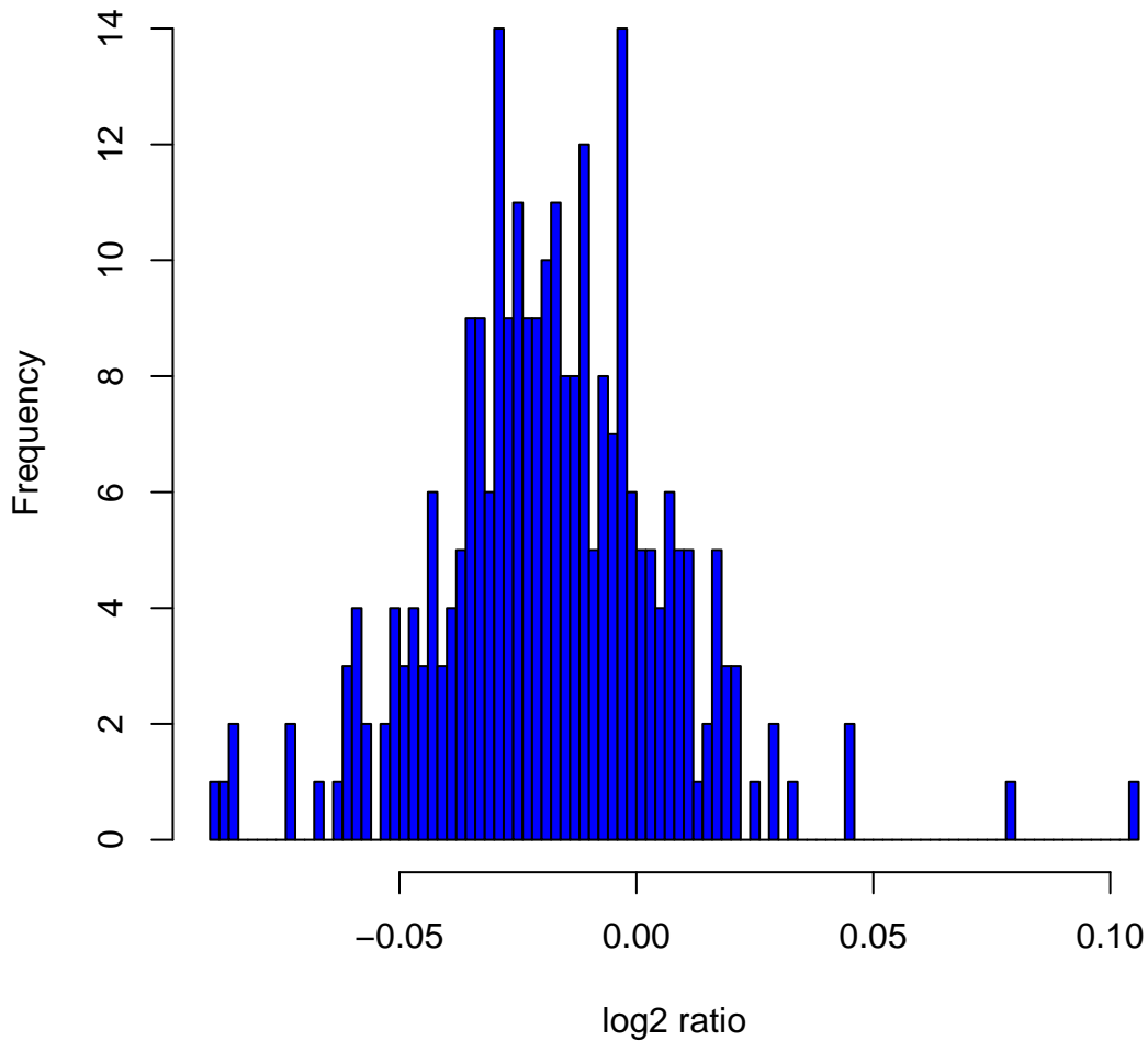
Histogram of log2ratios in 270 HapMap samples at clone Chr14tp-11C1
