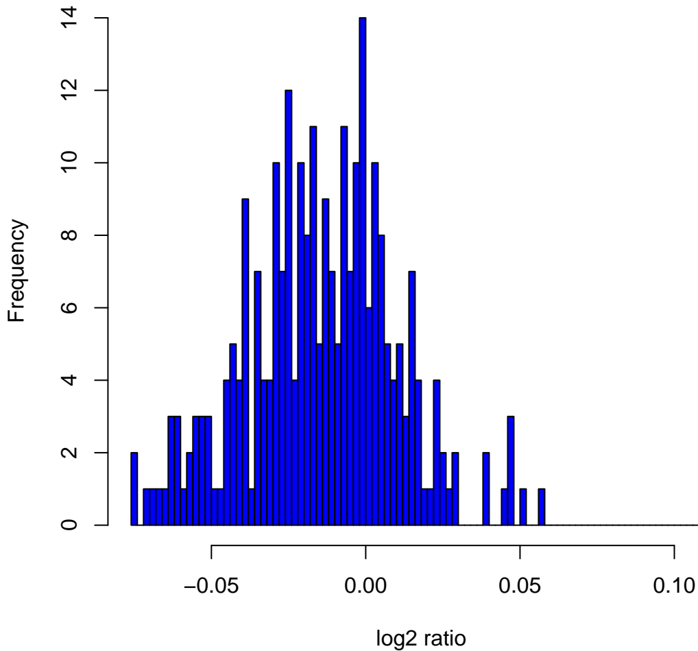
Histogram of log2ratios in 270 HapMap samples at clone Chr14tp-11C11
