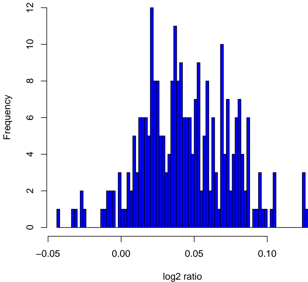
Histogram of log2ratios in 270 HapMap samples at clone Chr14tp-11C4
