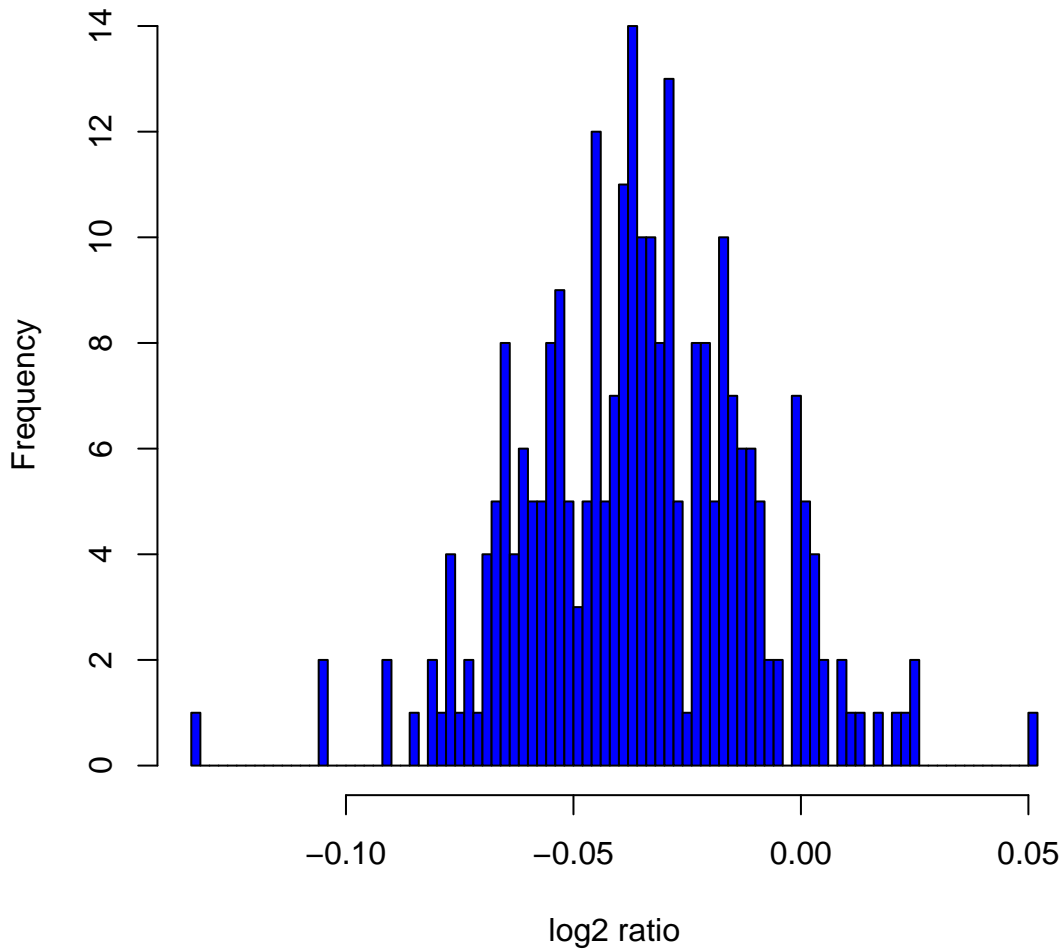
Histogram of log2ratios in 270 HapMap samples at clone Chr14tp-11D5
