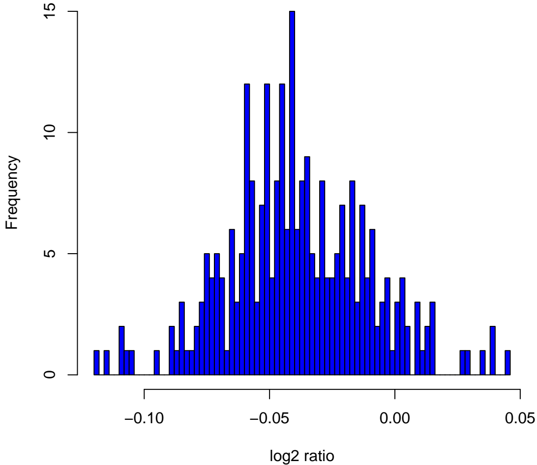
Histogram of log2ratios in 270 HapMap samples at clone Chr14tp-11E6
