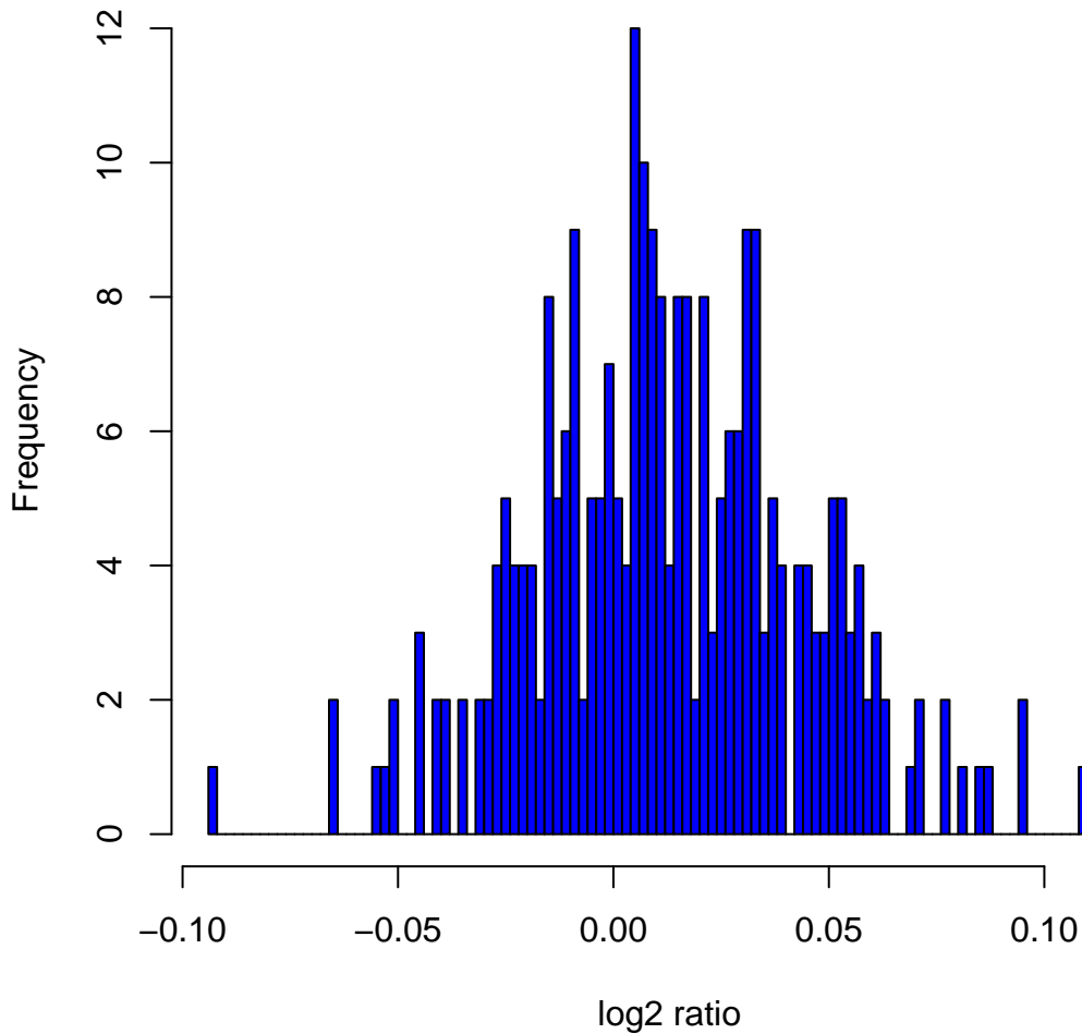
Histogram of log2ratios in 270 HapMap samples at clone Chr14tp-11G10
