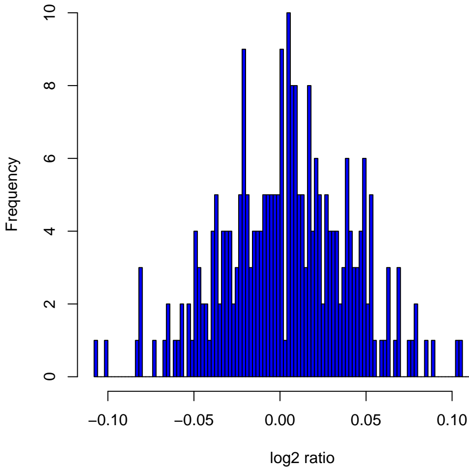
Histogram of log2ratios in 270 HapMap samples at clone Chr14tp-11H2
