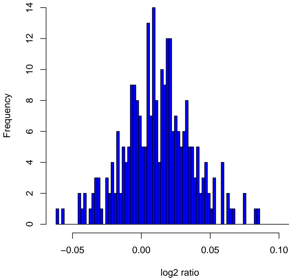
Histogram of log2ratios in 270 HapMap samples at clone Chr14tp-12D5
