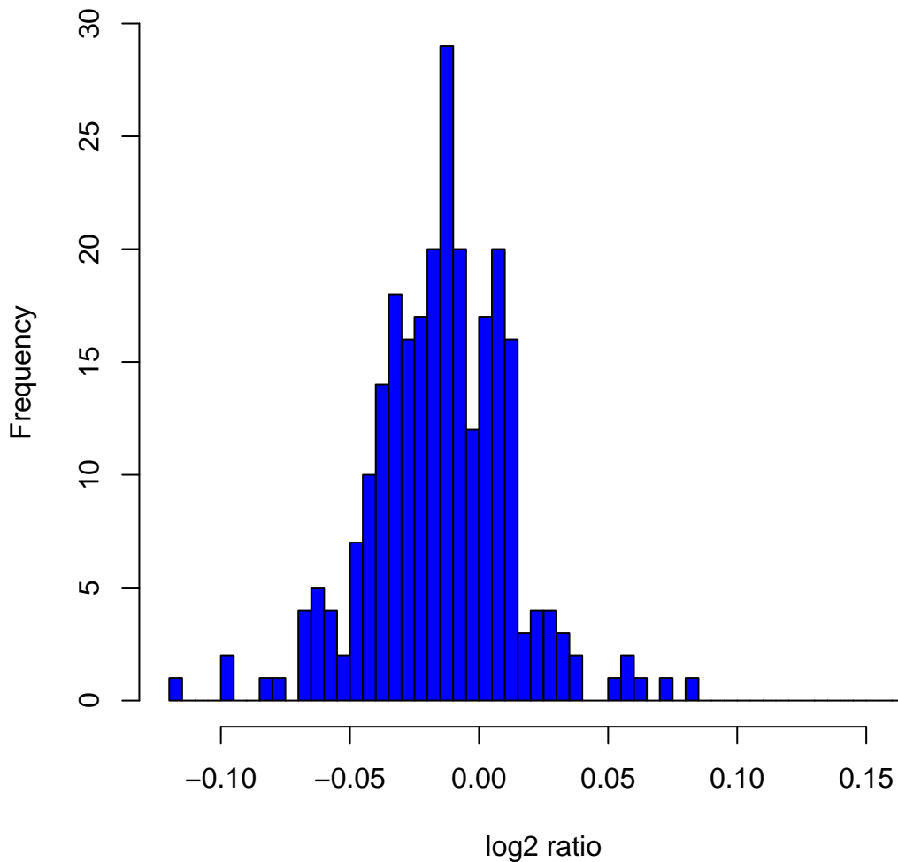
Histogram of log2ratios in 270 HapMap samples at clone Chr14tp-13A6
