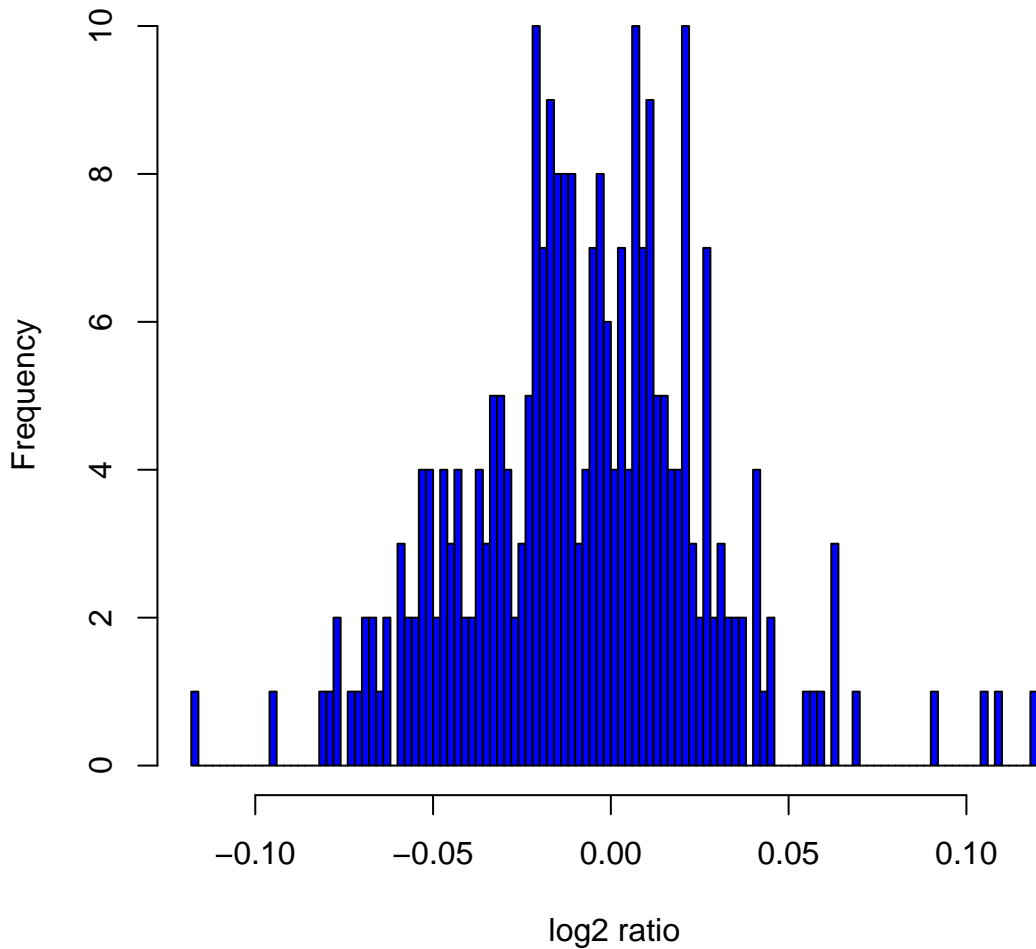
Histogram of log2ratios in 270 HapMap samples at clone Chr14tp-13B9
