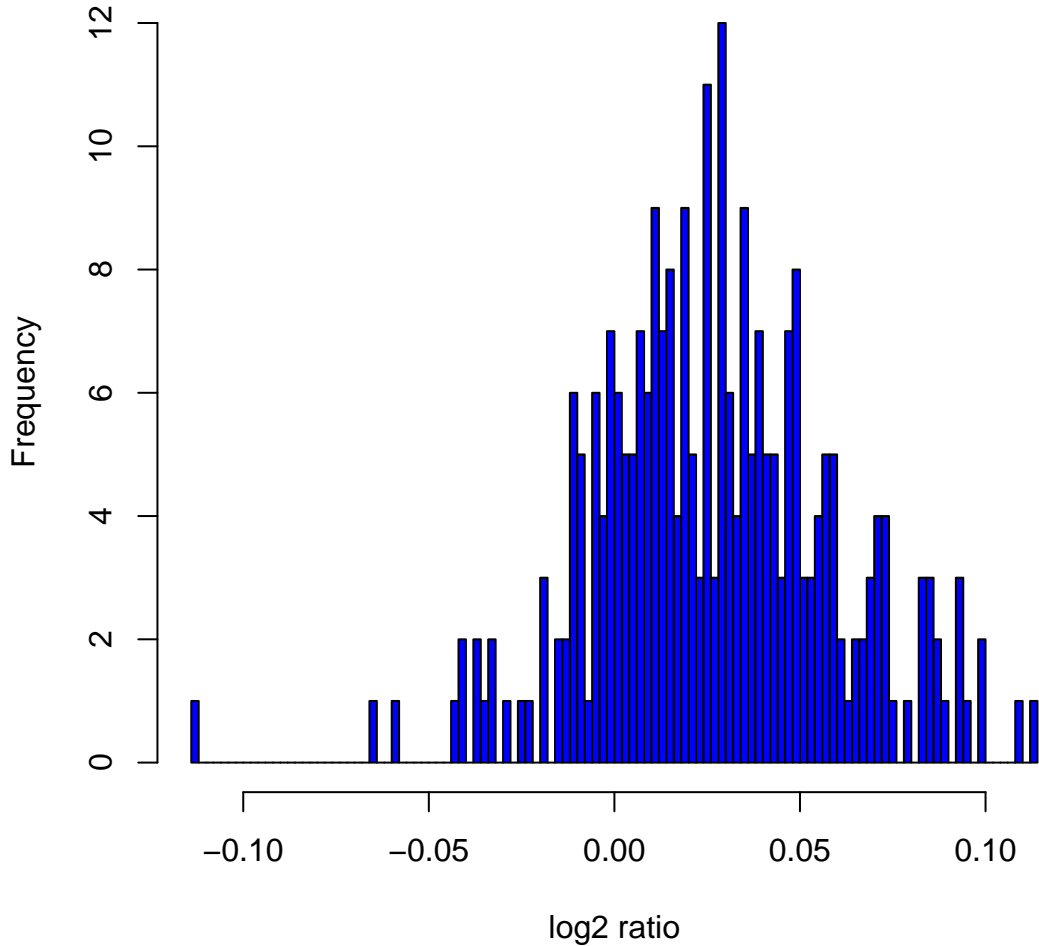
Histogram of log2ratios in 270 HapMap samples at clone Chr14tp-13C1
