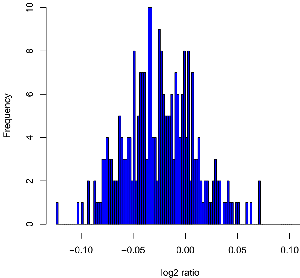
Histogram of log2ratios in 270 HapMap samples at clone Chr14tp-13C3
