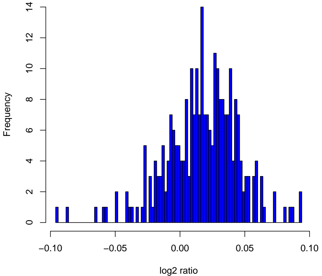
Histogram of log2ratios in 270 HapMap samples at clone Chr14tp-1A11
