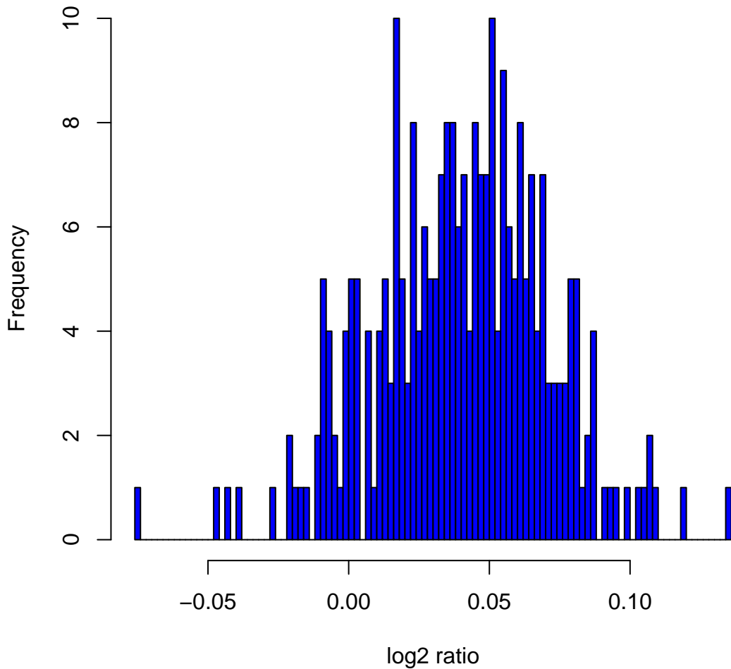
Histogram of log 2 ratios in 270 HapMap samples at clone Chr14tp-1C4
