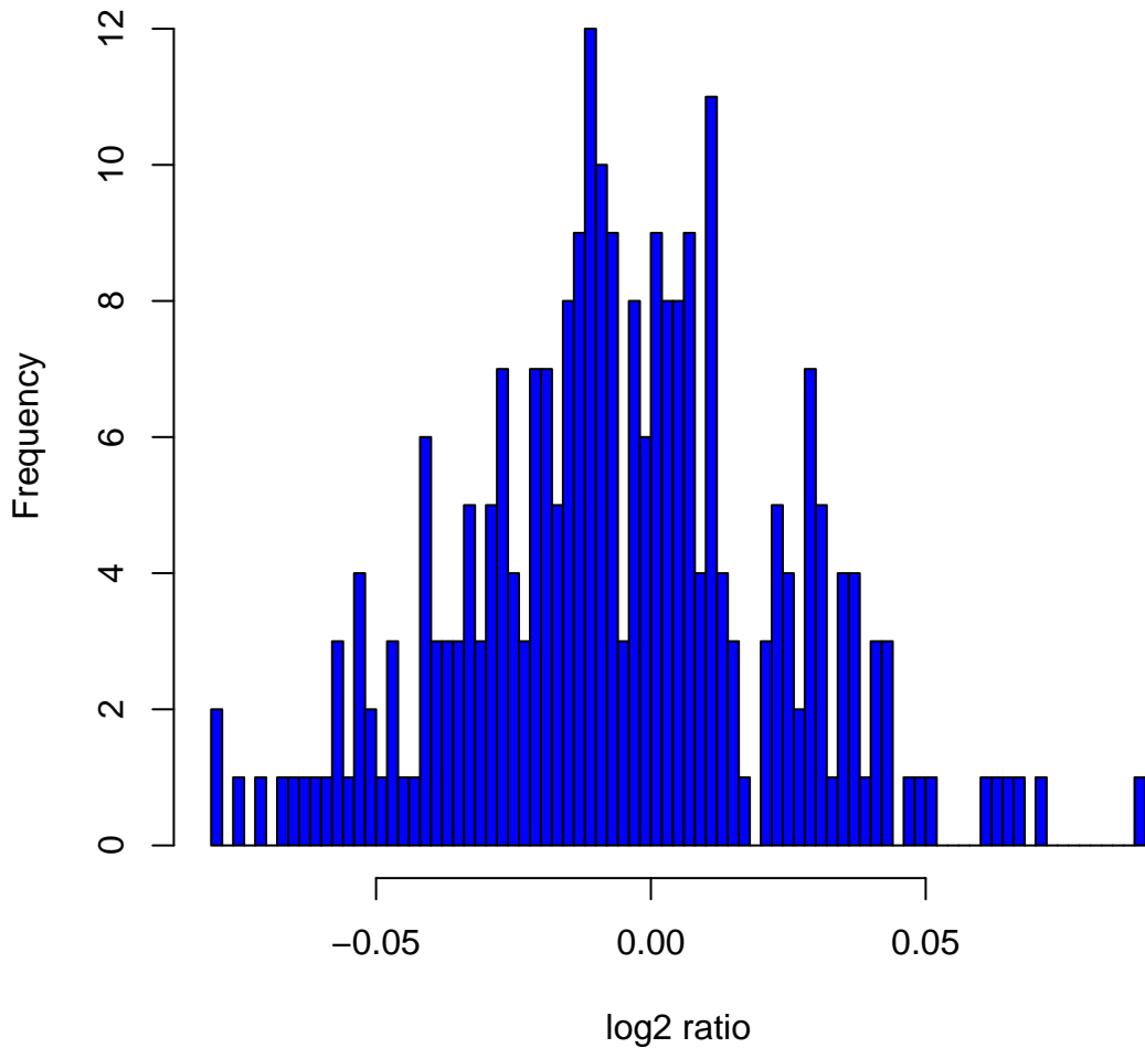
Histogram of log2ratios in 270 HapMap samples at clone Chr14tp-2B1
