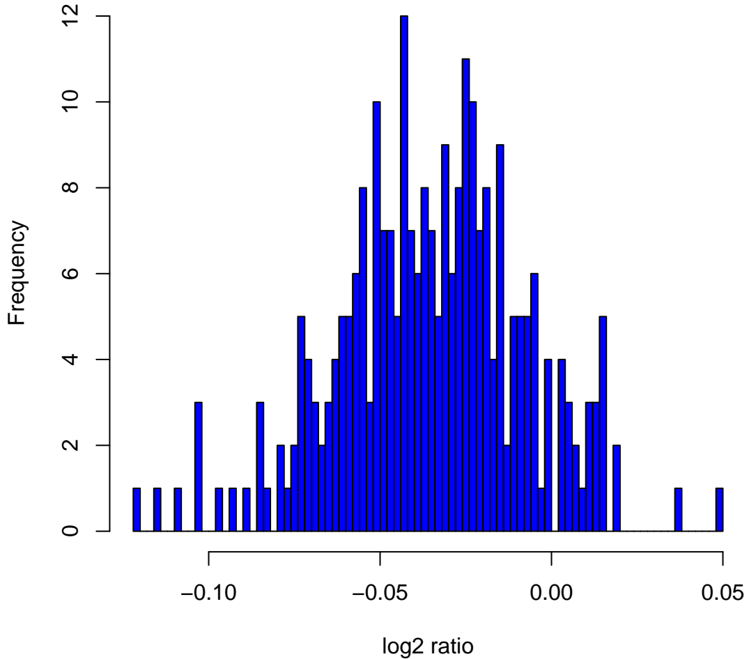
Histogram of log2ratios in 270 HapMap samples at clone Chr14tp-2E10
