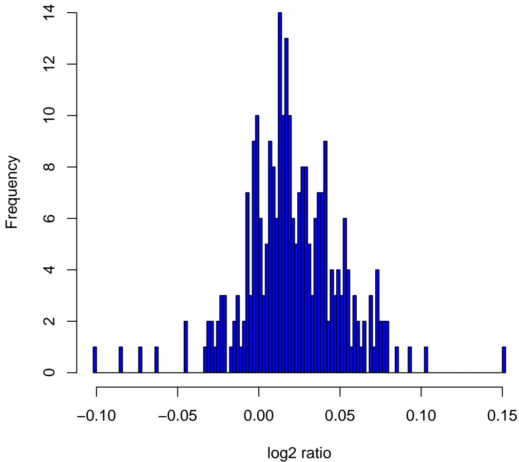
Histogram of log2ratios in 270 HapMap samples at clone Chr14tp-2G4
