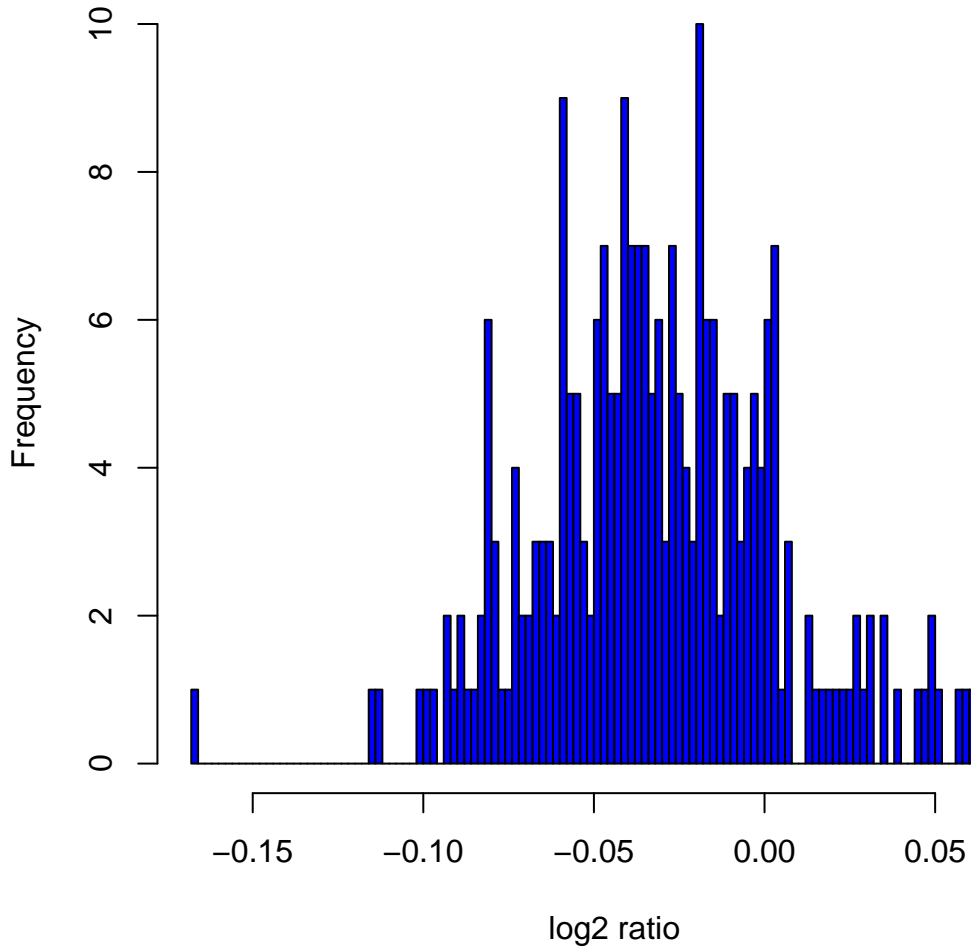
Histogram of log2ratios in 270 HapMap samples at clone Chr14tp-2H11
