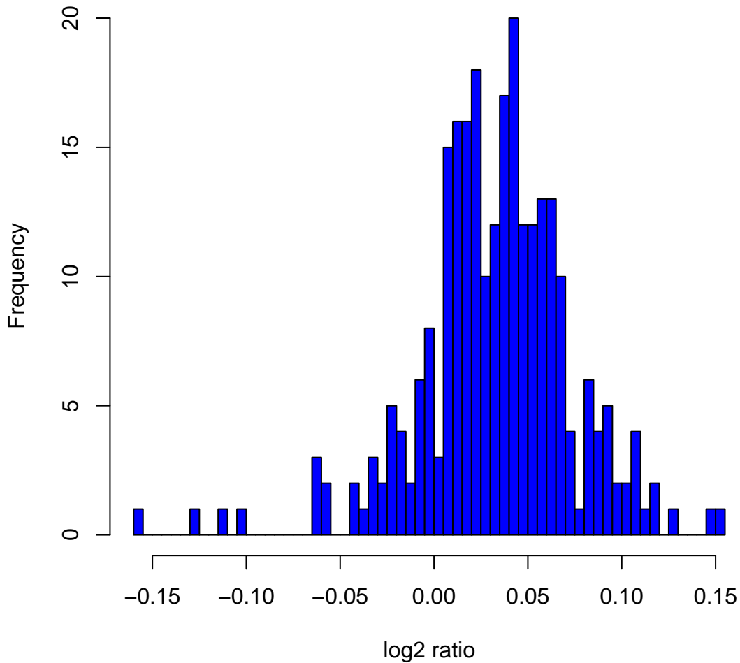
Histogram of log2ratios in 270 HapMap samples at clone Chr14tp-3A12
