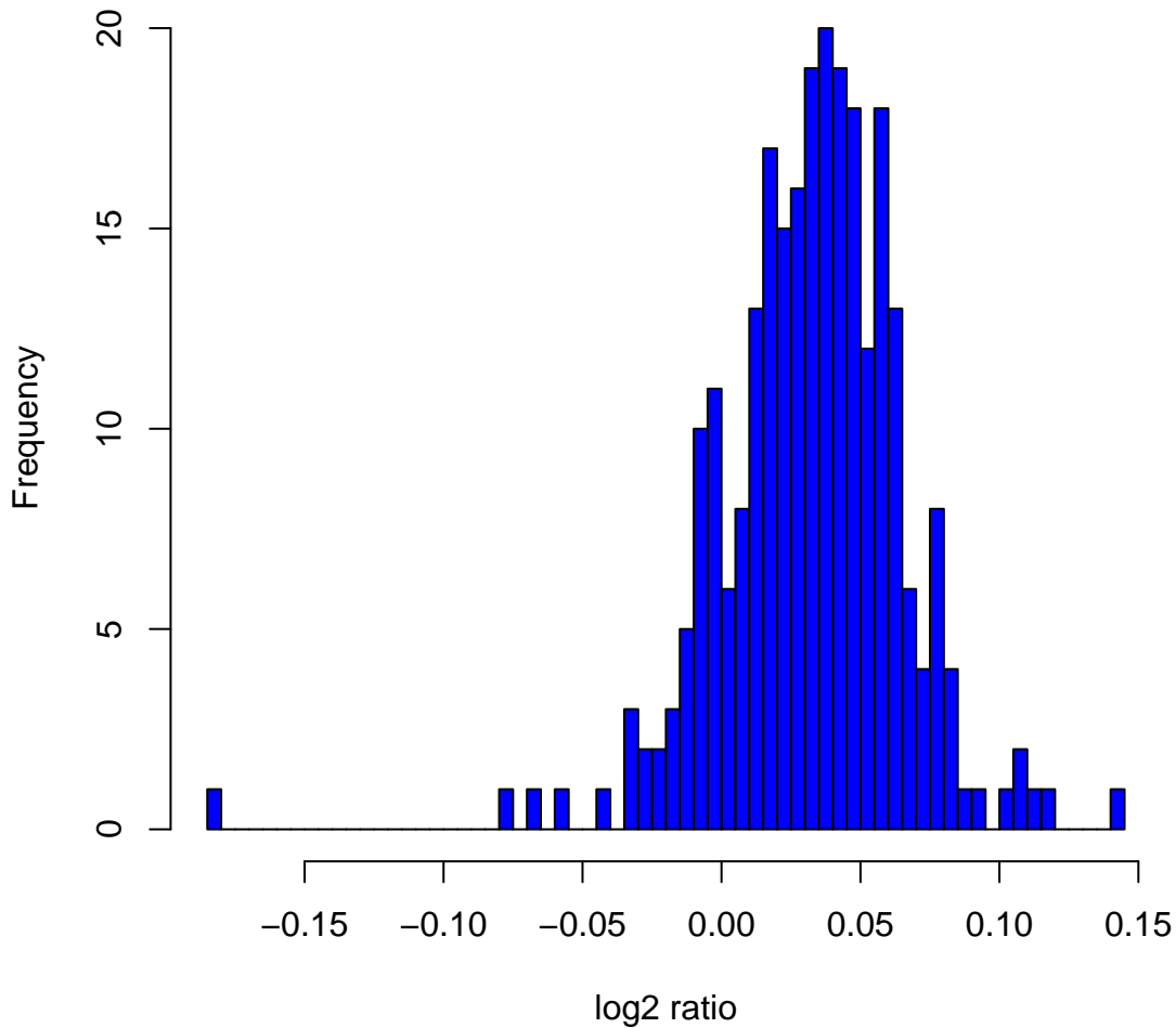
Histogram of log2ratios in 270 HapMap samples at clone Chr14tp-5A12
