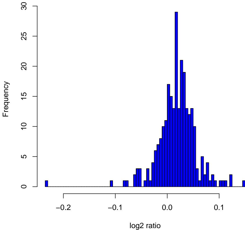
Histogram of log 2 ratios in 270 HapMap samples at clone Chr14tp-5A6
