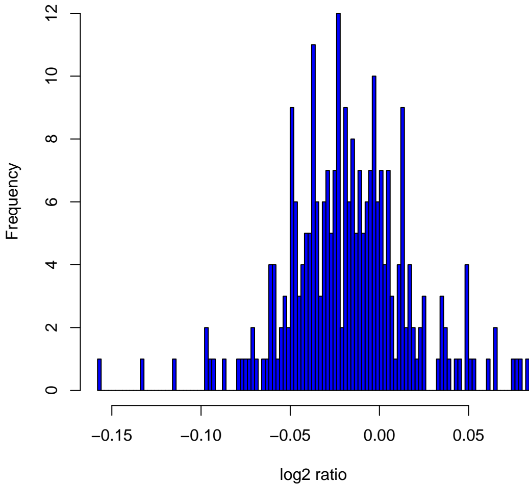
Histogram of log2ratios in 270 HapMap samples at clone Chr14tp-5G12
