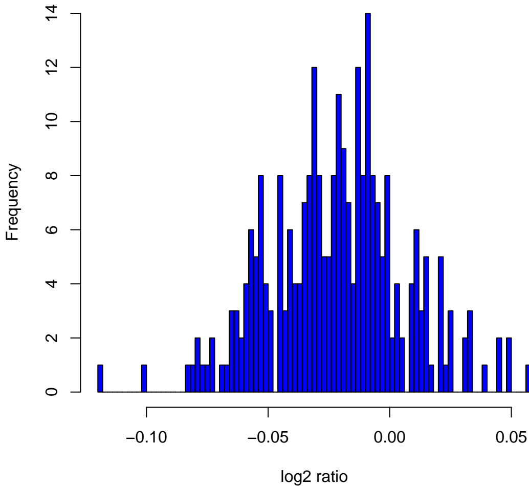
Histogram of log 2 ratios in 270 HapMap samples at clone Chr14tp-5G9
