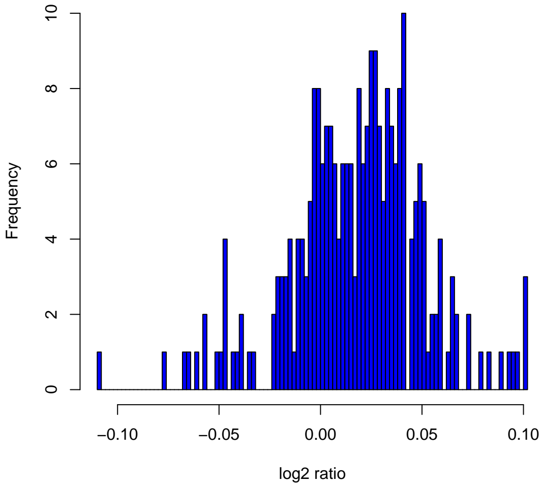
Histogram of log 2 ratios in 270 HapMap samples at clone Chr14tp-6D1
