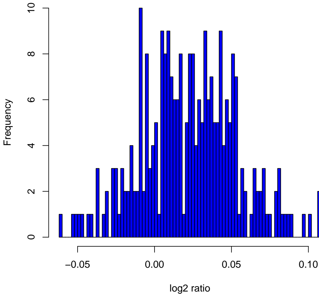
Histogram of log2ratios in 270 HapMap samples at clone Chr14tp-6D11
