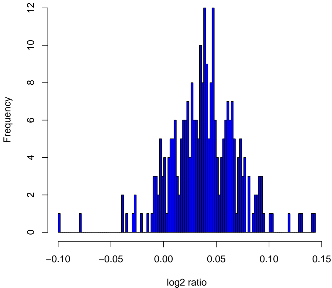
Histogram of log2ratios in 270 HapMap samples at clone Chr14tp-6D12
