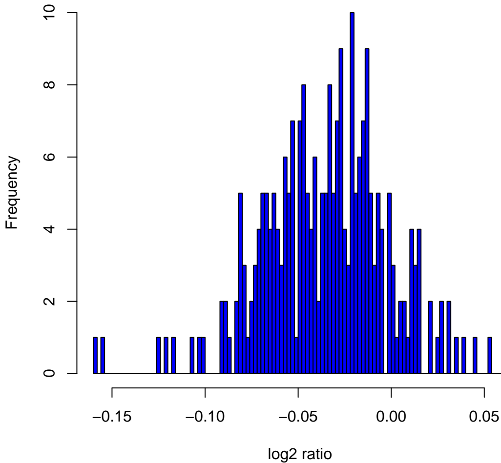
Histogram of log2ratios in 270 HapMap samples at clone Chr14tp-6D2
