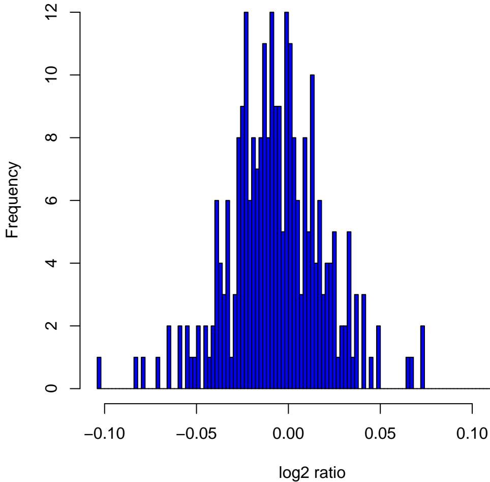
Histogram of \log_2 ratios in 270 HapMap samples at clone Chr14tp-6G9
