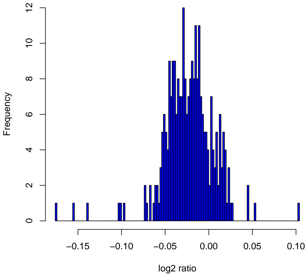
Histogram of log 2 ratios in 270 HapMap samples at clone Chr14tp-7A3
