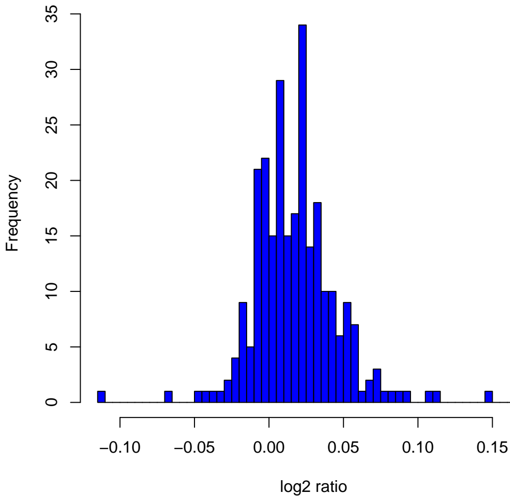
Histogram of log 2 ratios in 270 HapMap samples at clone Chr14tp-8C5
