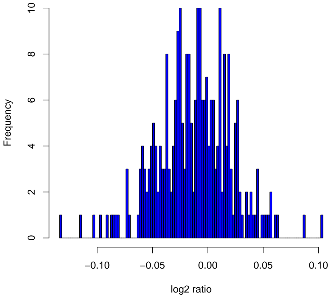
Histogram of log 2 ratios in 270 HapMap samples at clone Chr14tp-8D7
