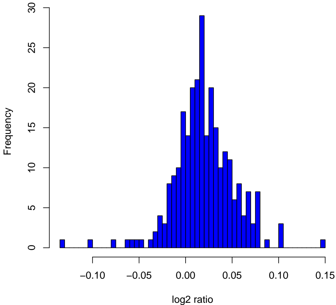
Histogram of log2ratios in 270 HapMap samples at clone Chr14tp-8D9
