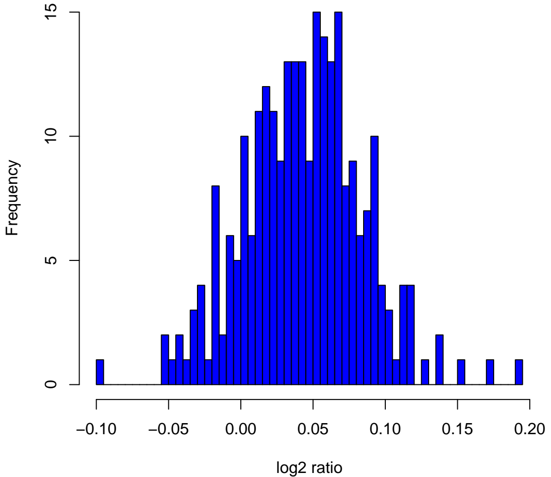
Histogram of log2ratios in 270 HapMap samples at clone Chr15tp-10B1
