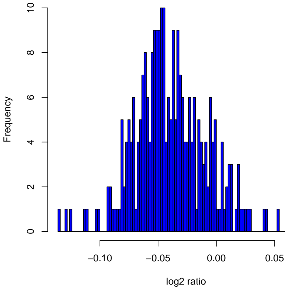
Histogram of log2ratios in 270 HapMap samples at clone Chr15tp-10C8
