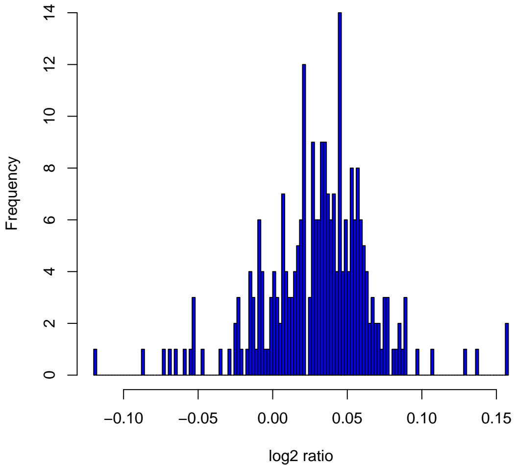
Histogram of log2ratios in 270 HapMap samples at clone Chr15tp-10E9
