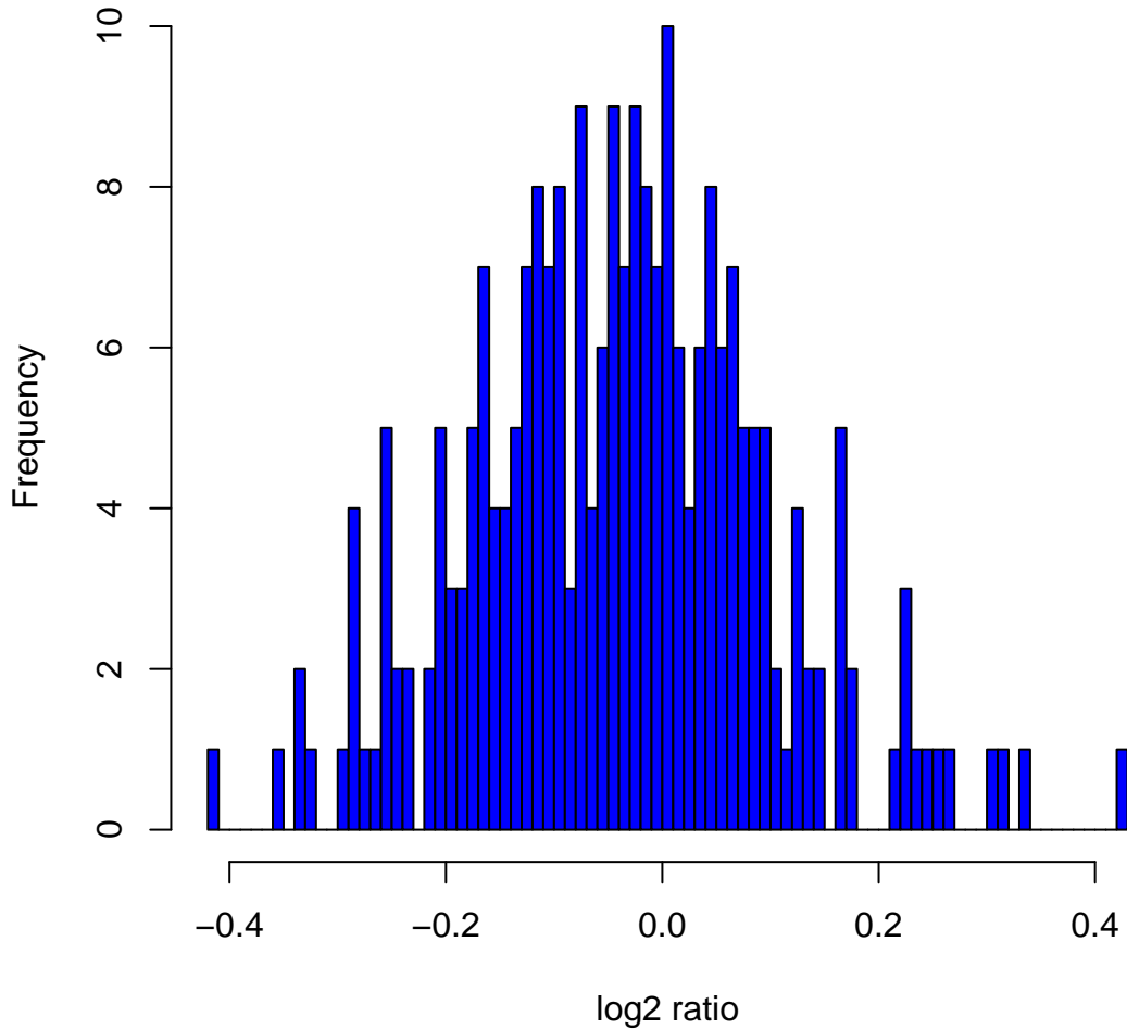
Histogram of log2ratios in 270 HapMap samples at clone Chr15tp-10F4
