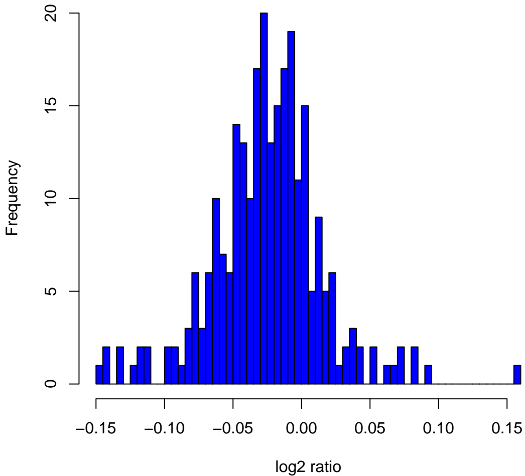
Histogram of log2ratios in 270 HapMap samples at clone Chr15tp-11H9
