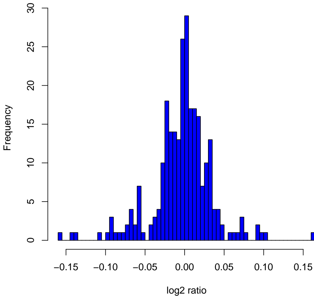
Histogram of log2ratios in 270 HapMap samples at clone Chr15tp-1F11
