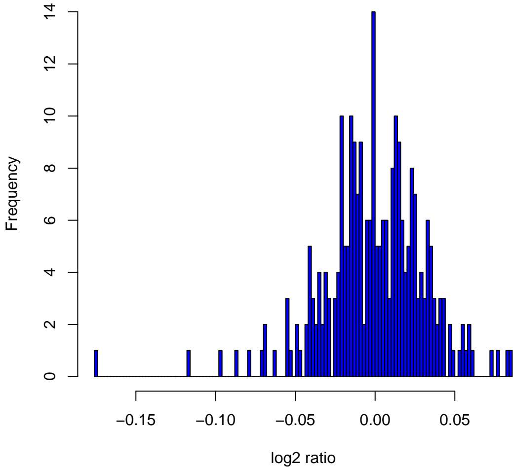
Histogram of log2ratios in 270 HapMap samples at clone Chr15tp-2A11
