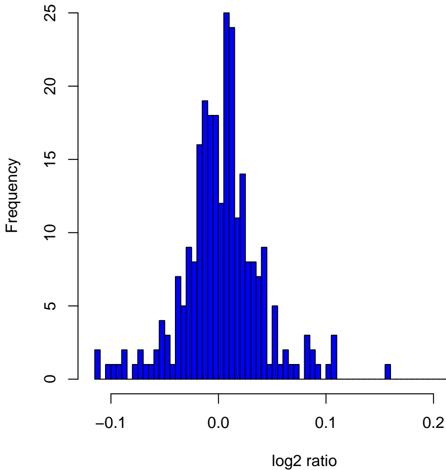
Histogram of log2ratios in 270 HapMap samples at clone Chr15tp-2C10
