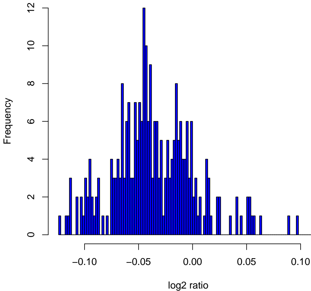
Histogram of log 2 ratios in 270 HapMap samples at clone Chr15tp-3A6
